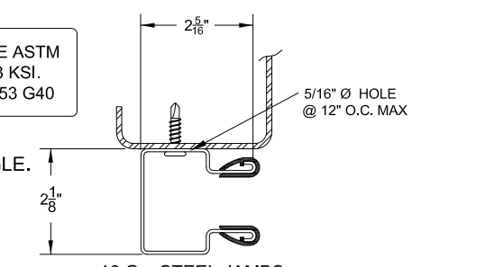
16 Ga. STEEL JAMBS USING #12-14 X 1" TEKS PANCAKE HEAD 16 GA (0.054" MIN) GUIDE MOUNTING DETAIL
