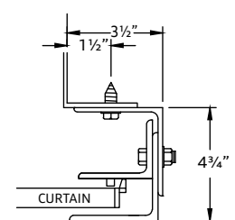
3 piece Structural Steel Windload Certified Guide
