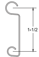
22 GAUGE STAINLESS STEEL FLAT SLAT
