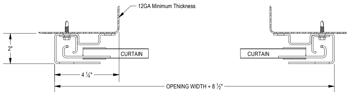
FIGURE 9: STEEL JAMBS
