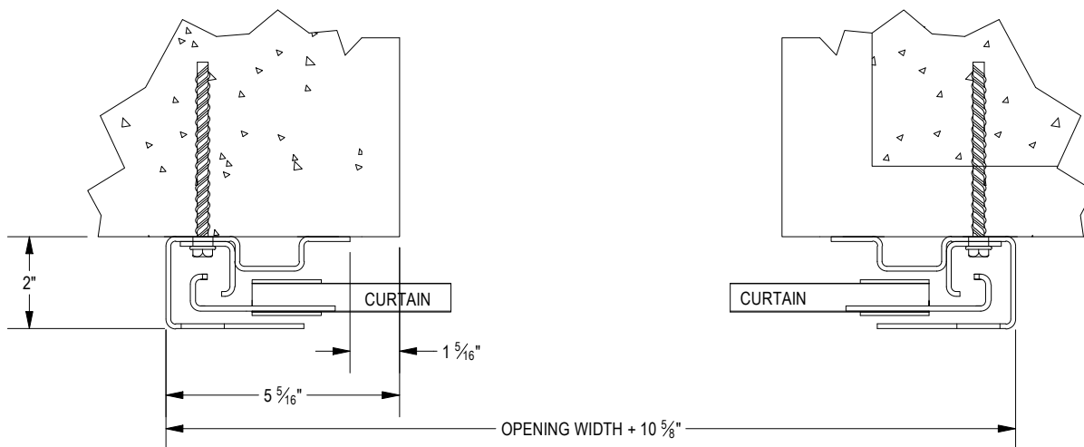
FIGURE 8: CONCRETE/FILLED CMU
