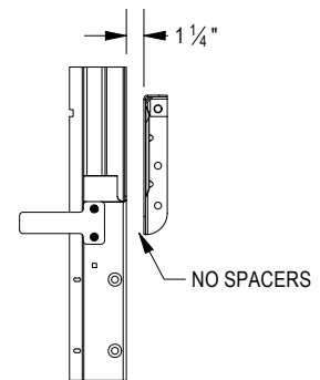
GUIDE / BRACKET SPACING
