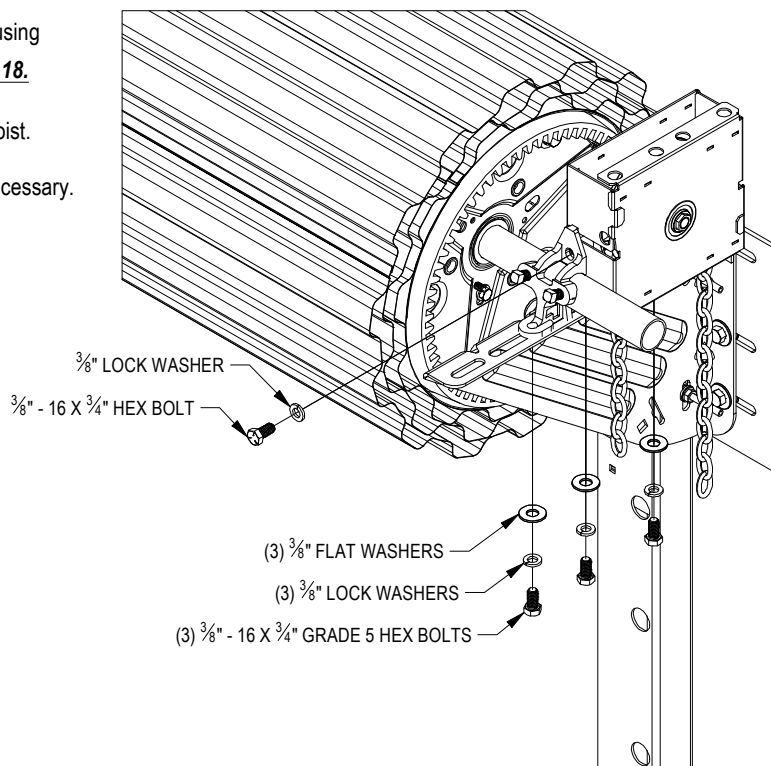
FIGURE 18: REDUCED HAND CHAIN DRIVE END
