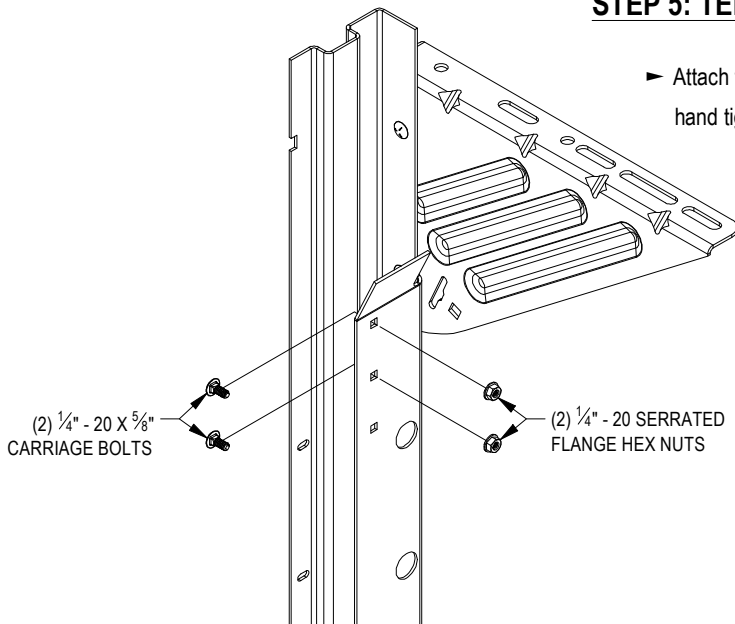
FIGURE 12: PRE INSTALL CARRIAGE BOLTS
