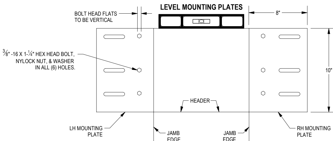
FIGURE 5: LARGE MOUNTING PLATE
