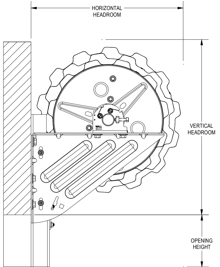
FIGURE 3: SIDEROOM CLEARANCE REQUIREMENT
