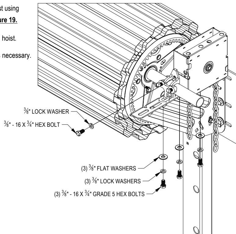
FIGURE 19: REDUCED HAND CHAIN DRIVE END
