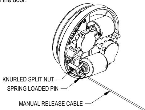
PANTHEON DRIVE UNIT
