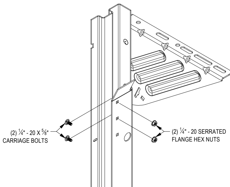
FIGURE 12: PRE INSTALL CARRIAGE BOLTS
