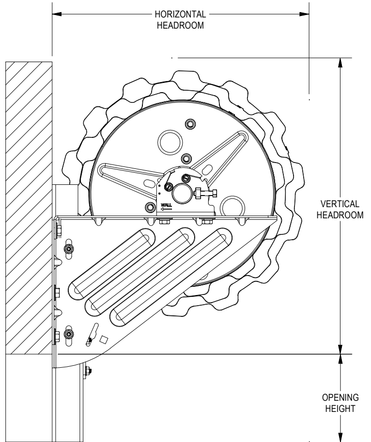
FIGURE 3: SIDE ROOM CLEARANCE REQUIREMENTS
