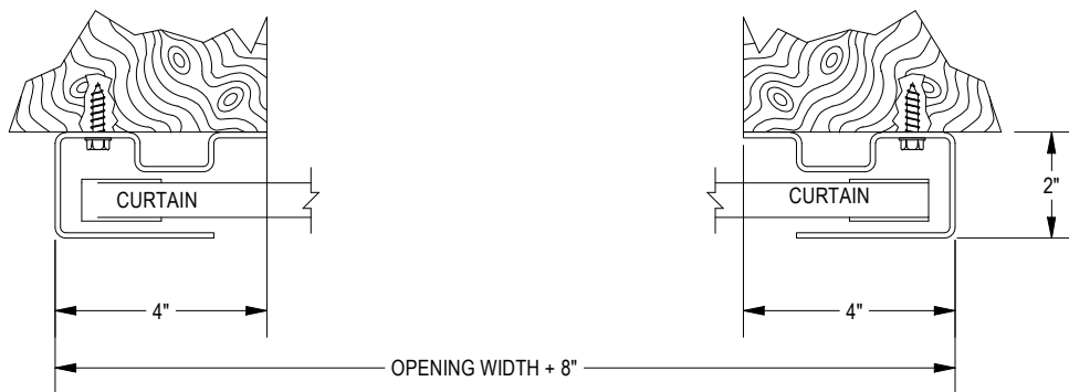
FIGURE 10: WOOD JAMBS
