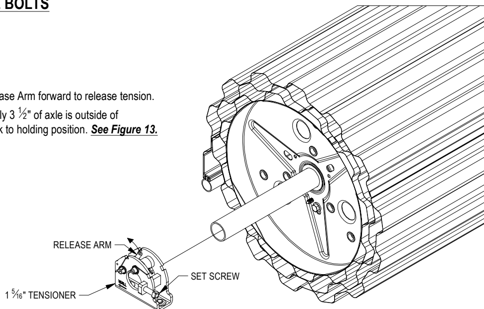
FIGURE 13: TENSIONER END
