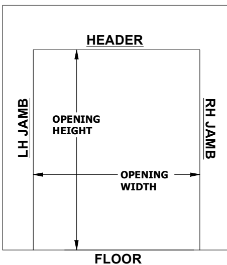
FIGURE 4: WALL OPENING
