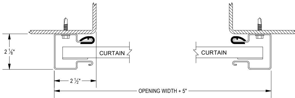
FIGURE 8: STEEL JAMBS
