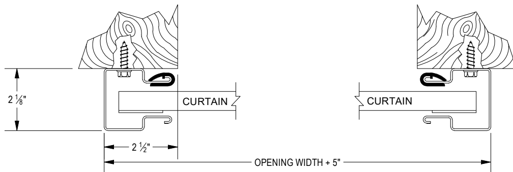
FIGURE 10: WOOD JAMBS
