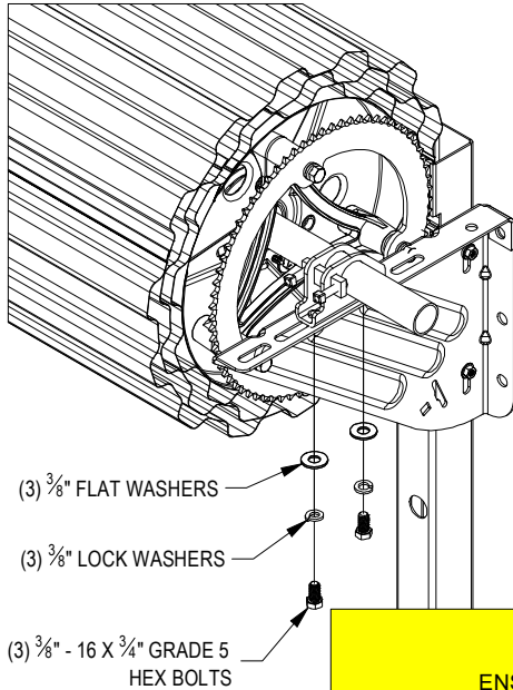
FIGURE 20: ELECTRIC DRIVE END
