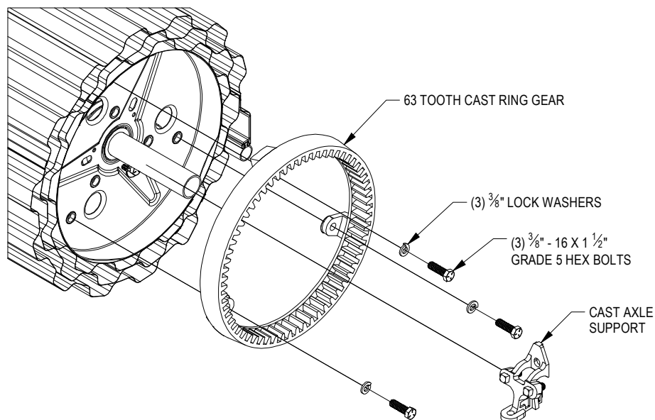
FIGURE 15: REDUCED CHAIN DRIVE END
