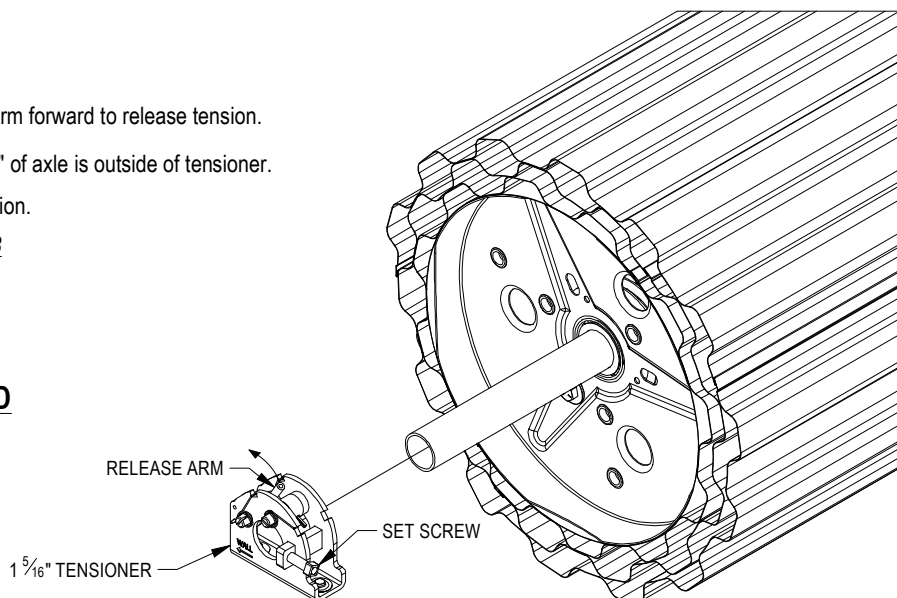
FIGURE 12: HEADSTOP PRE-INSTALLATION
