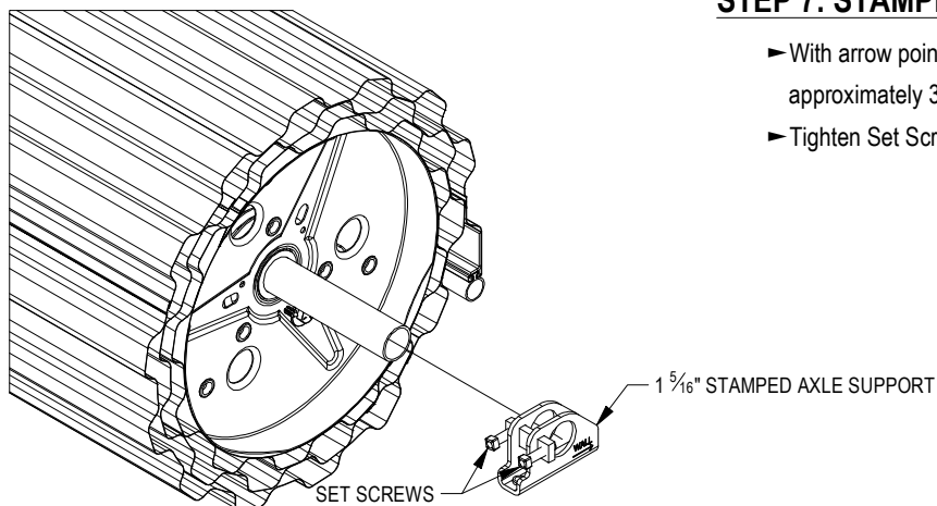
FIGURE 14: STAMPED AXLE SUPPORT END
