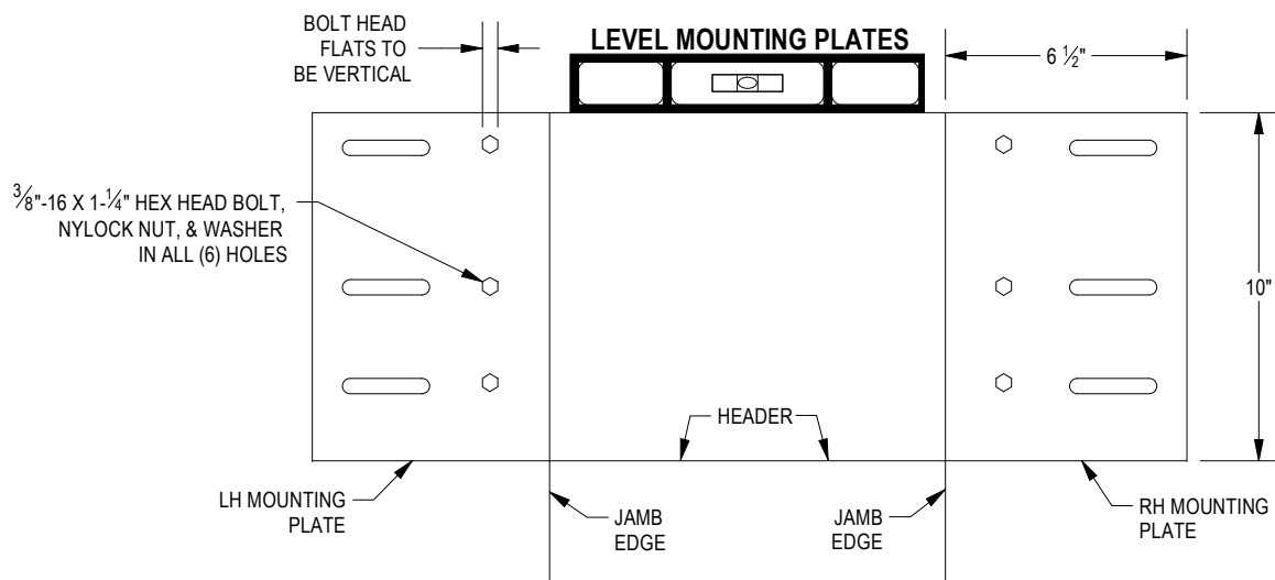
FIGURE 5: SMALL MOUNTING PLATES
