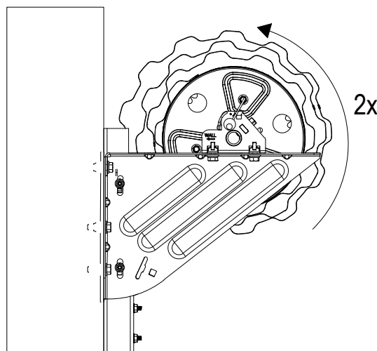
FIGURE 21: SETTING INITIAL SPRING TENSION
