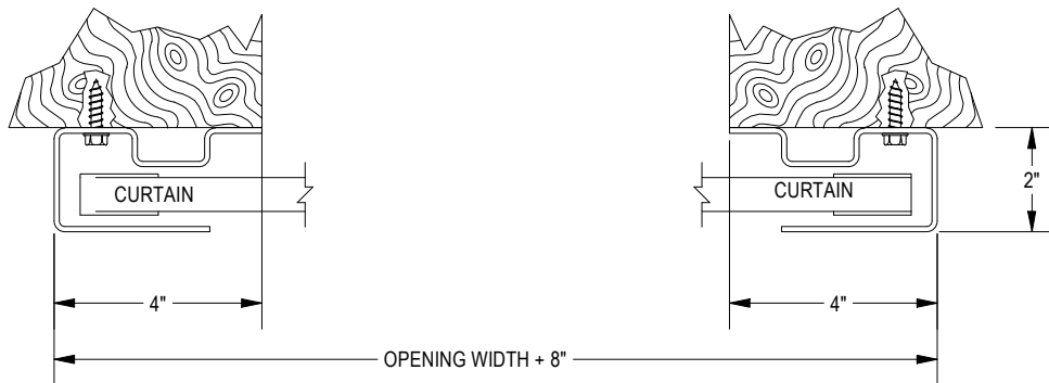
FIGURE 10: WOOD JAMBS
