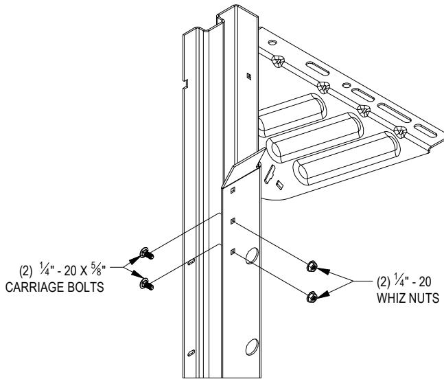
FIGURE 12: PRE INSTALL CARRIAGE BOLTS
