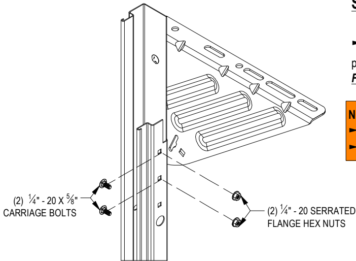
FIGURE 12: PRE INSTALL CARRIAGE BOLTS
