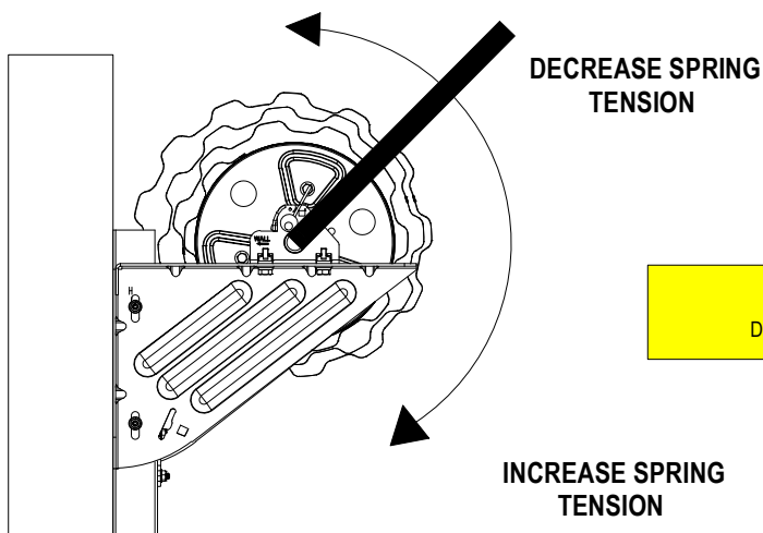
FIGURE 24: ADJUSTING SPRING TENSION
