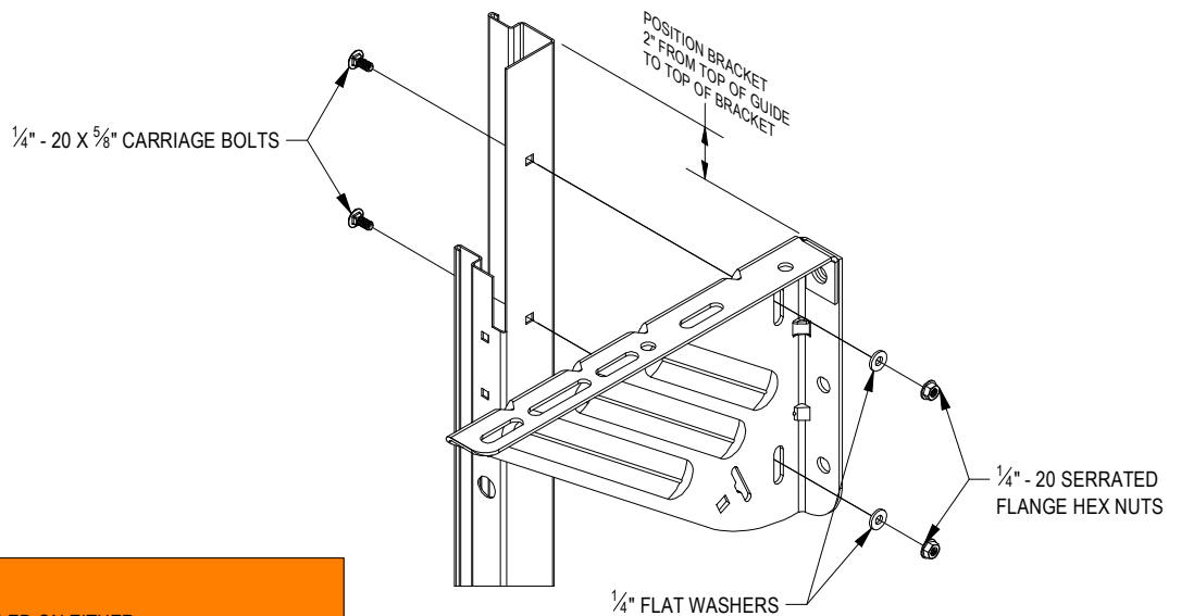
FIGURE 6: COMMERCIAL BRACKETS TO GUIDE
