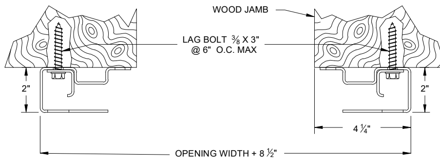
FIGURE 10: WOOD JAMBS
