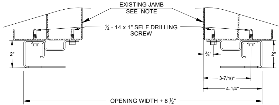
FIGURE 8: CONCRETE & FILLED MASONRY JAMBS
