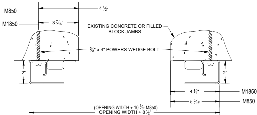
FIGURE 8: CONCRETE & FILLED MASONRY JAMBS
