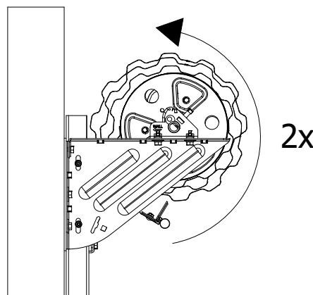
FIGURE 20: SETTING INITIAL SPRING TENSION
