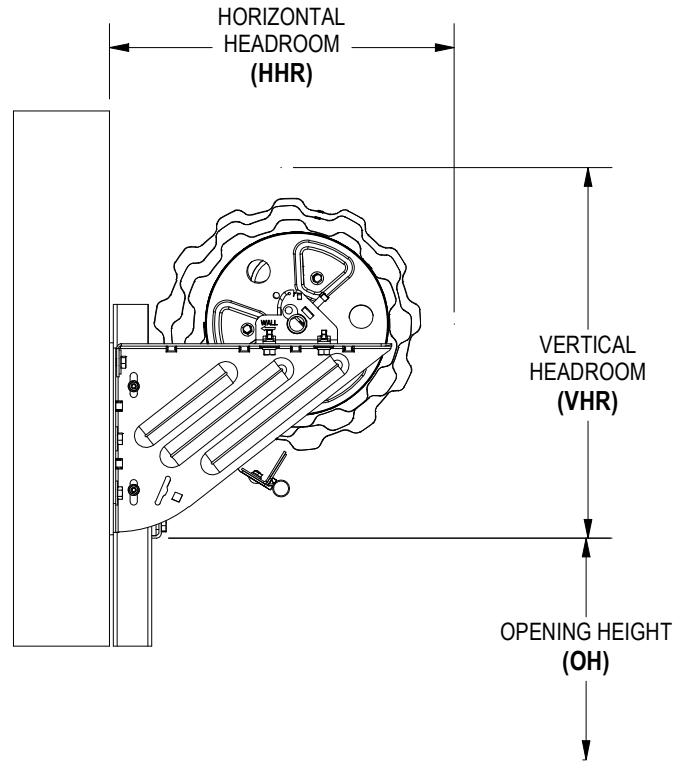
FIGURE 3: SIDE ROOM CLEARANCE REQUIREMENT CHART
