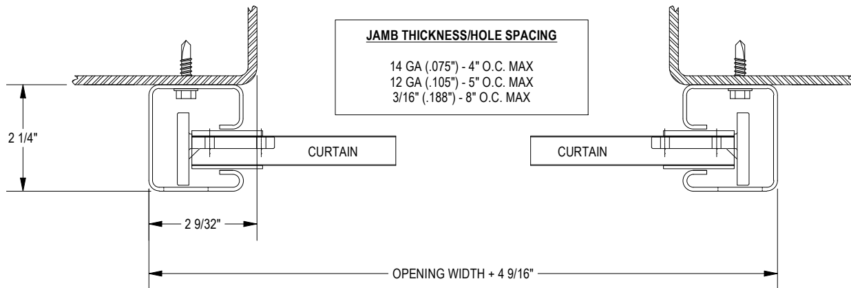
FIGURE 9: STEEL JAMBS
