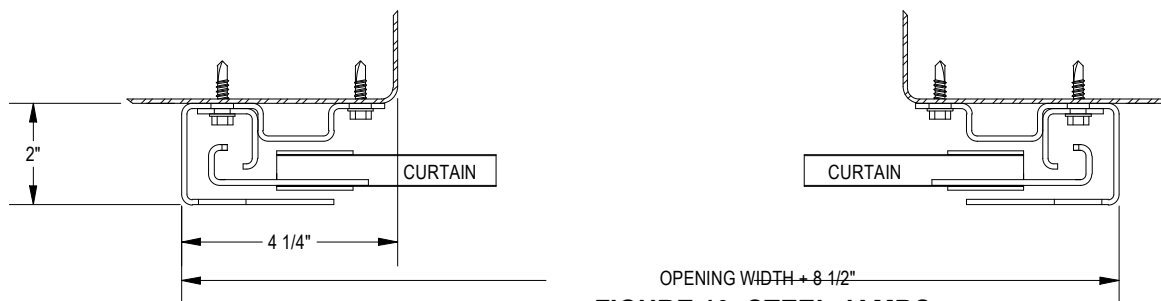
FIGURE 10: STEEL JAMBS
