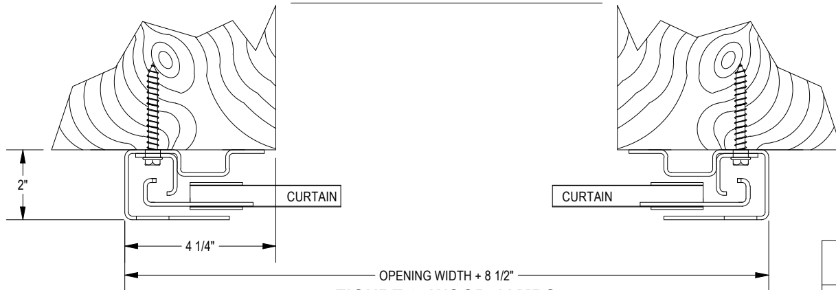
FIGURE 9: WOOD JAMBS
