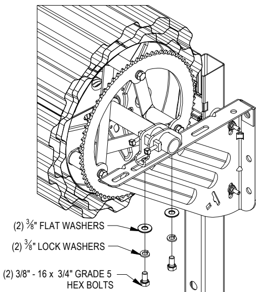
FIGURE 20: ELECTRIC DRIVE END
