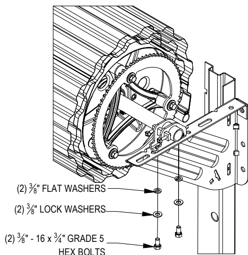
FIGURE 18: ELECTRIC DRIVE END
