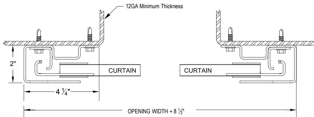
FIGURE 9: STEEL JAMBS
