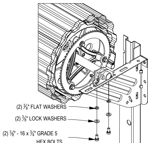
FIGURE 19: ELECTRIC DRIVE END
