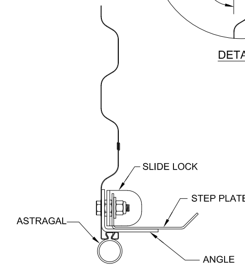
BOTTOM BAR ASSEMBLY
