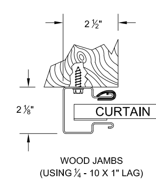
16 GA GUIDE MOUNTING DETAIL
