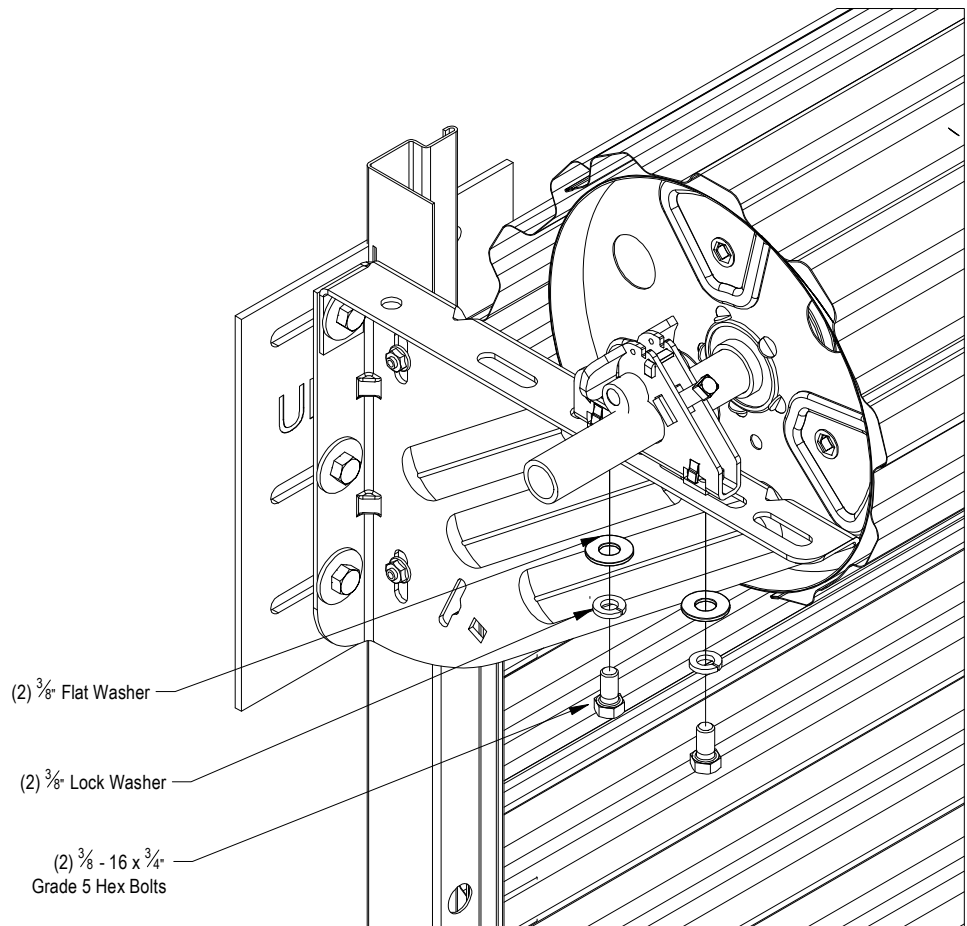
FIGURE 16: TENSIONER END
