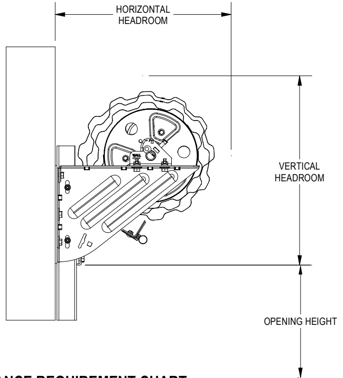
FIGURE 3: SIDE ROOM CLEARANCE REQUIREMENT CHART
