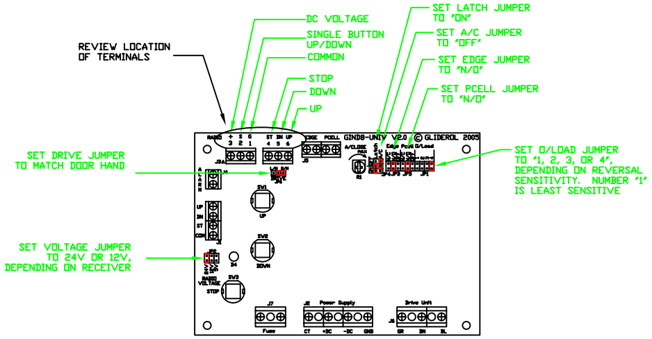
RADIO RECEIVER CONNECTIONS AND JUMPER SETTINGS
