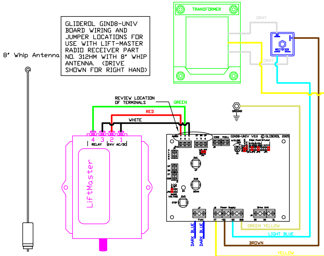
RADIO RECEIVER CONNECTIONS AND JUMPER SETTINGS
