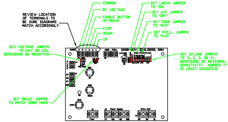
RADIO RECEIVER CONNECTIONS AND JUMPER SETTINGS
